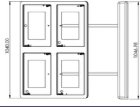
Claralight™ 4 panel frame dimensions
